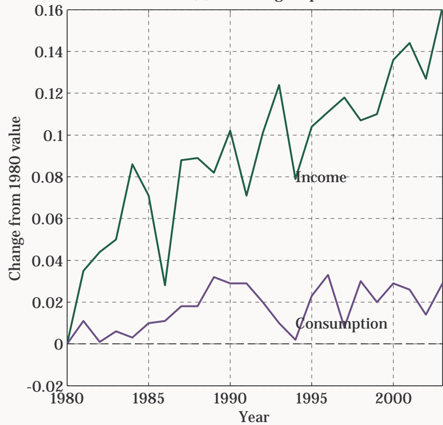
(b) Within-group
